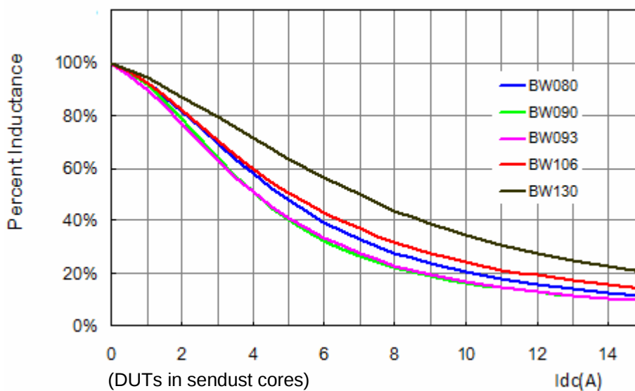
Inductance v.s. DC Bias
