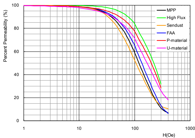
DC-bias property at 25°C
