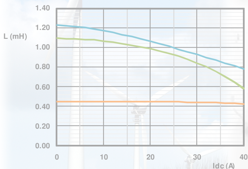
DC BIAS CHARACTERISTICS
